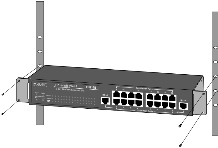
Figure 2-11 Rack Mounting
