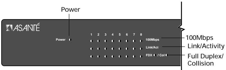
Figure 3-2 FS4008DS LEDs
